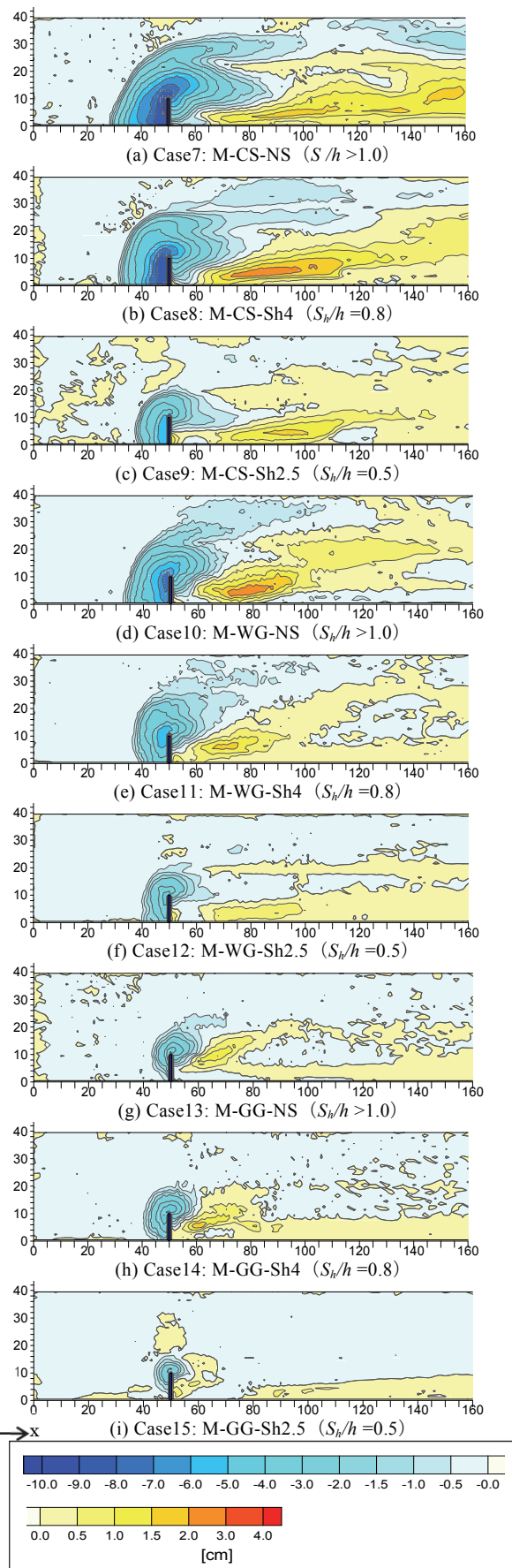
Fig. 11 Bed contour at the quasi-equilibrium stage for non-uniform sediment bed
