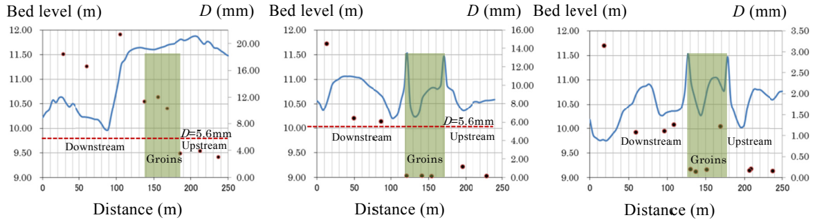
Fig.7 Bed level (lines) and mean sediment sizes (points) along longitudinal sections L1, L2 and L3 (Left: Section-L1; Middle: Section L2; Right: Section L3)
