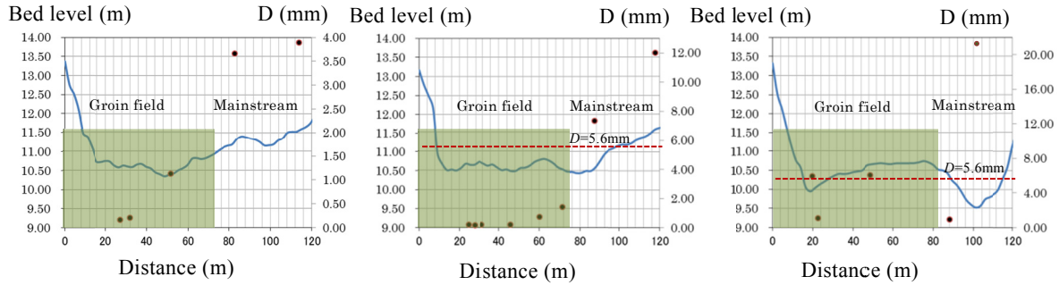
Fig.9 Bed level (lines) and mean sediment sizes (points) along transverse sections T1, T2 and T3 (Left: Section-T1; Middle: Section-T2; Right: Section-T3)
